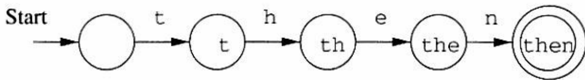
Figure 1.2: A finite automaton modeling recognition of then
