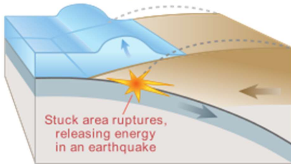
Tsunami starts during earthquake
