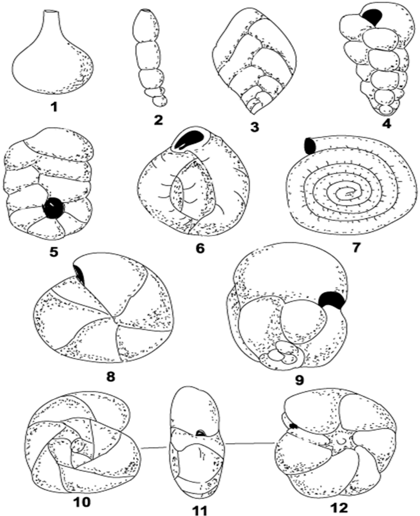
Principle types of chamber arrangement. 1, single chambered; 2, uniserial; 3, biserial; 4, triserial; 5, planispiral to biserial; 6, milioline; 7, planispiral evolute; 8, planispiral involute; 9, streptospiral; 10-11-12,
